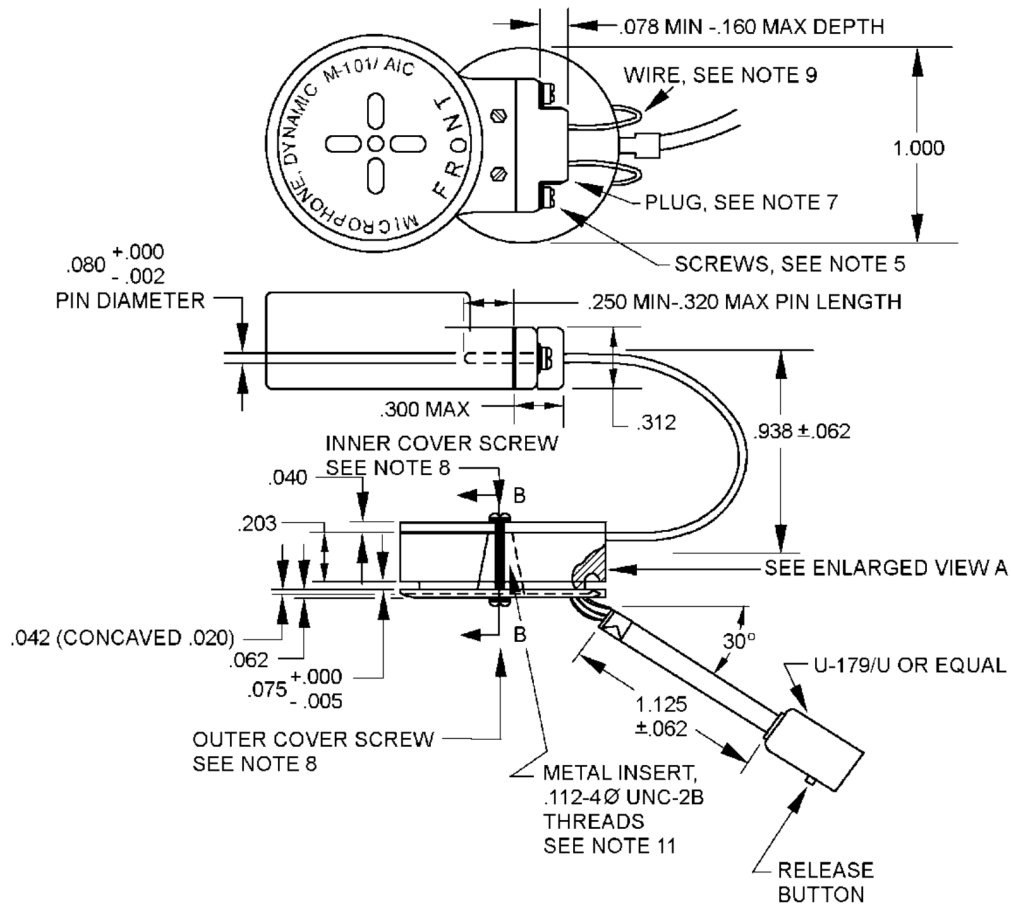
FIGURE 1. Microphone assembly, M100/AIC.
